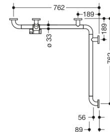
Abmessungen in mm
